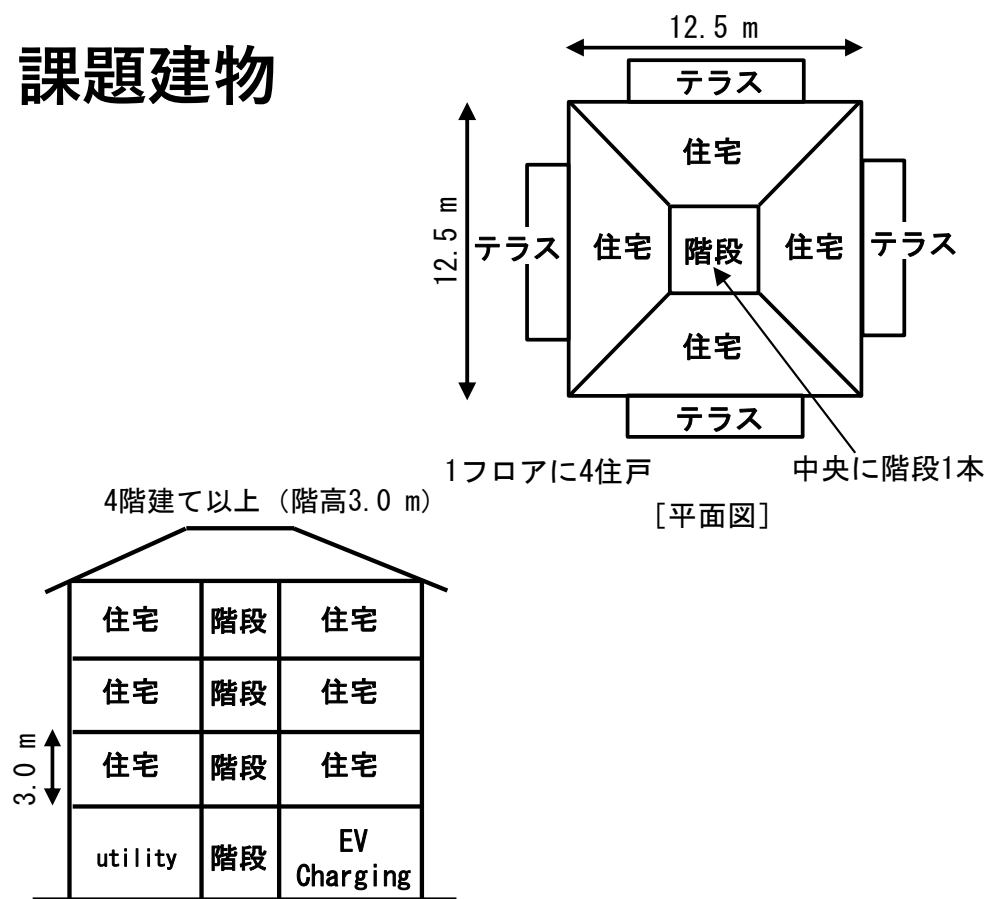
[断面図]
